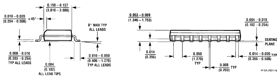
16-Lead (0.150" Wide) Small Outline Integrated Circuit, SOIC JEDEC Package Number M16A
